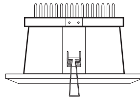
ILLUCEO 156mm 9 LED 3000K 700mA
